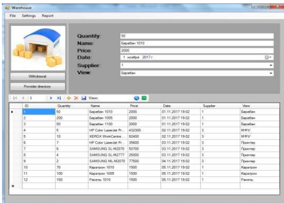
Picture 5. Warehouse
